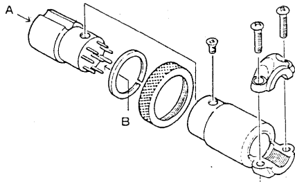
Plug assembly
