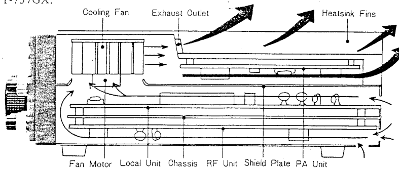
FT-757GX Duct Flow Cooling System
